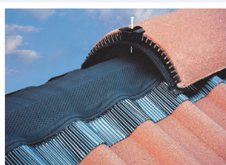
FOR ADDITIONAL HIGH VENTILATION Dry Fix Rollout Ridge and Hip Product Code: HD ROR & HD CON
